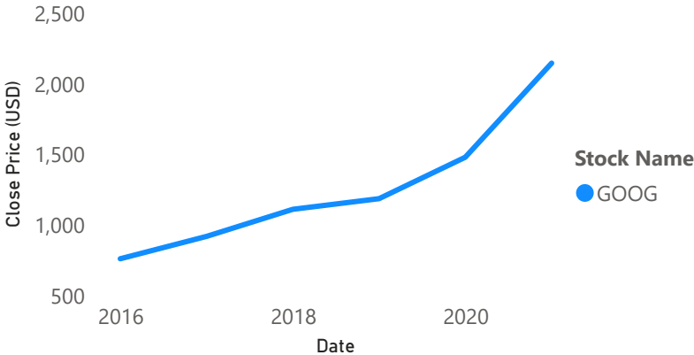
GOOG Price Trend (2016–2021)
